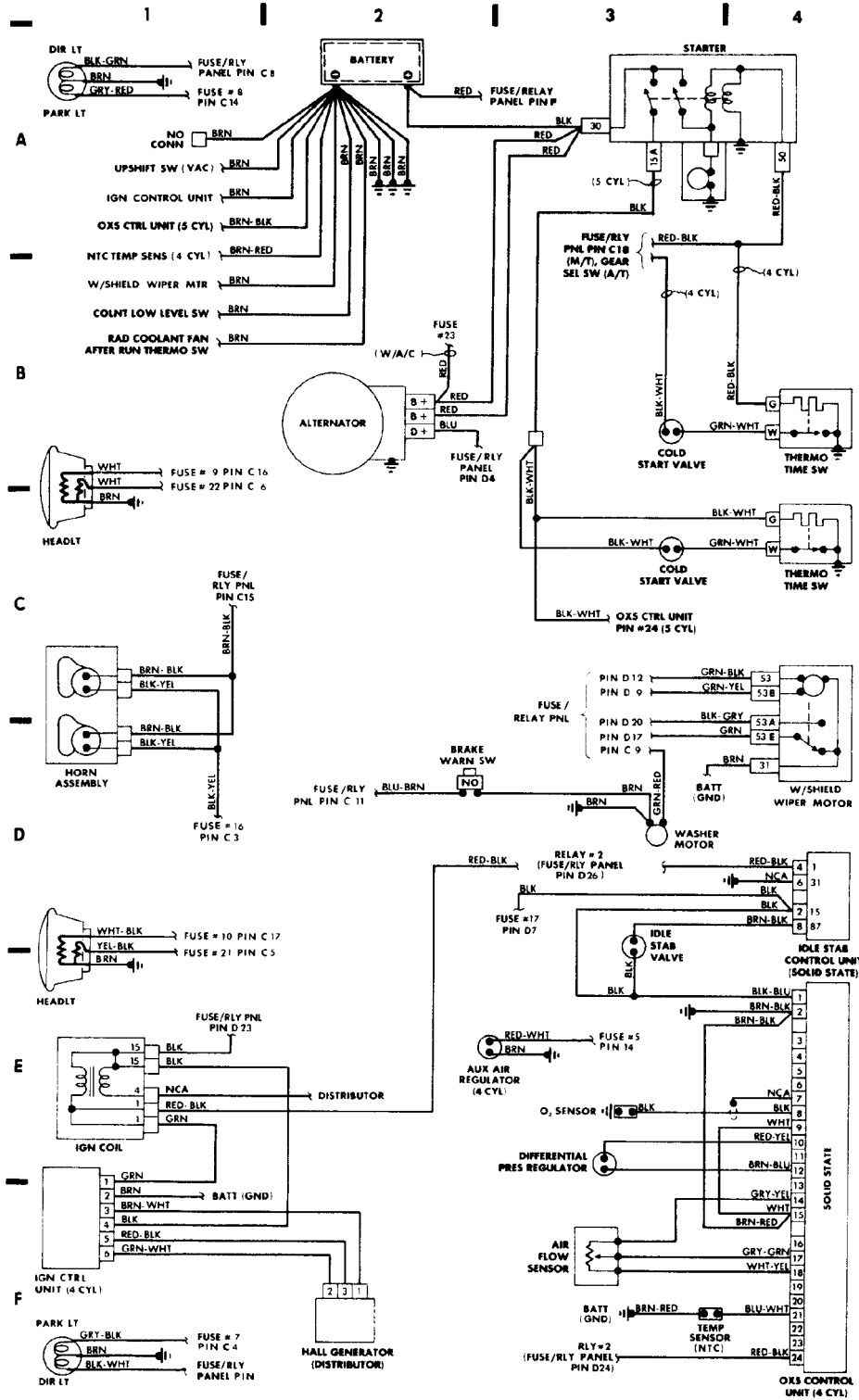
Fig. 1: Engine Compartment (Grids 1-4)
