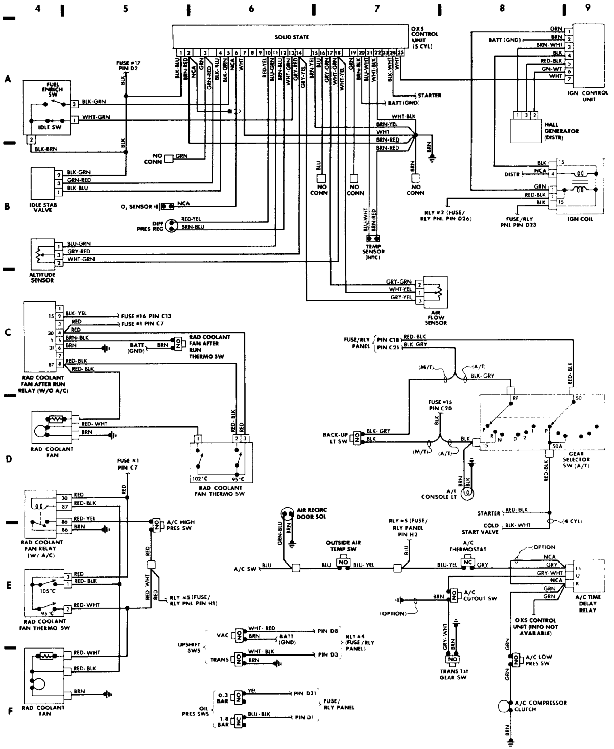
Fig. 2: Engine Compartment (Cont.) & Underdash (Grids 4-9)
