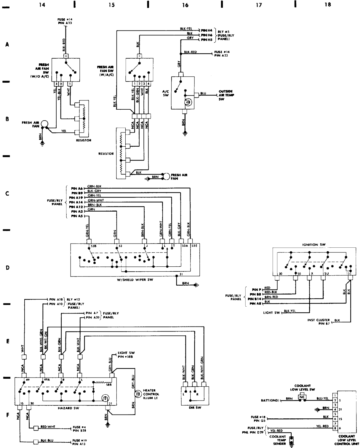
Fig. 4: Underdash (Cont.) & Instrument Panel (Grids 14-18)
