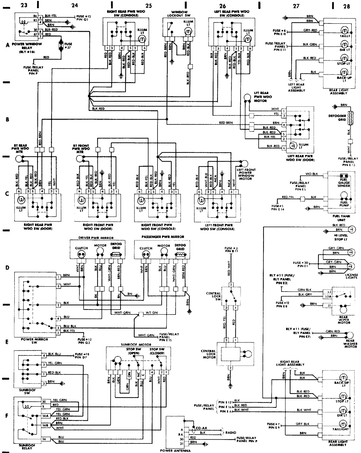
Fig. 6: Rear Compartment (Cont.) & Accessories (Grids 23-28)
