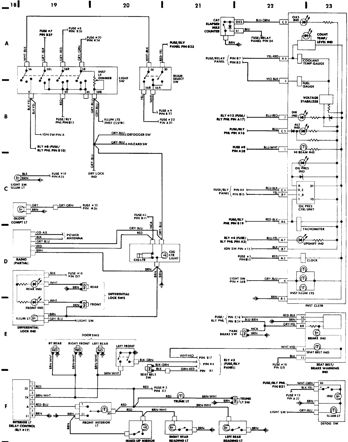
Fig. 5: Instrument Panel (Cont.) & Rear Compartment (Grids 18-23)
